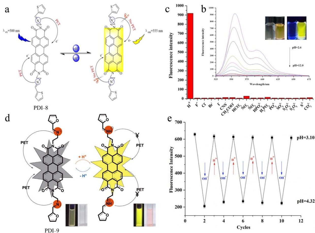
Figure 7. (a) Scheme of PET-based pH sensing mechanism of PDI-8 probe; (b) pH-sensitive fluorescence spectra of PDI-8 (10 \mu\text{M} ) in DMF/HEPES ( v/v , 4/1) buffer solution and the corresponding photographs taken under daylight (left) and UV light (right), respectively; (c) Selectivity test of the fluorescence response of PDI-8 toward \text{H}^+ compared to other anions (50 \mu\text{M} , pH = 2.6) in DMF/HEPES ( v/v , 4/1) buffered aqueous solution. Reproduced with permission from Ref [15]. (d) Scheme of PET-based pH sensing mechanism of PDI-9 and pH-sensitive color change under UV light (left) and daylight (right), respectively; (e) Reversibility of the fluorescence intensity modulation tested for PDI-9 between pH 4.32 and 3.10. Reproduced with permission from Ref [13].
