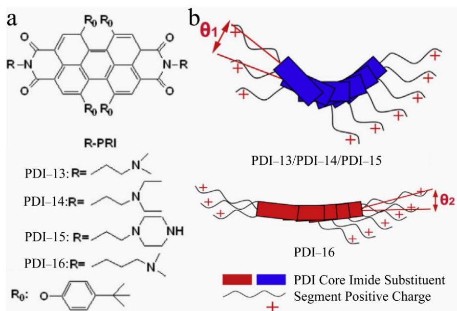
Figure 10. (a) Molecular structures of PDI-13/14/15/16 and (b) proposed self-assembly scheme for the nanofibers formed upon protonation. Reproduced with permission from Ref [17].
