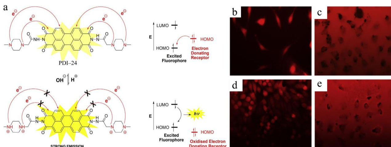
Figure 15. (a) Molecular structure of PDI-24 and its photophysical mechanism for pH probing; (b–e) Fluorescent photographs (under bars of 50 \mu\text{m} ) of PDI-24 micelles in living L929 cells. The cells were incubated for 24 h (upper) and 48 h (lower) with PDI-24 concentrations of 1.3 \mu\text{M} (b,d) and 26 \mu\text{M} (c,e). Reproduced with permission from Ref [23].
