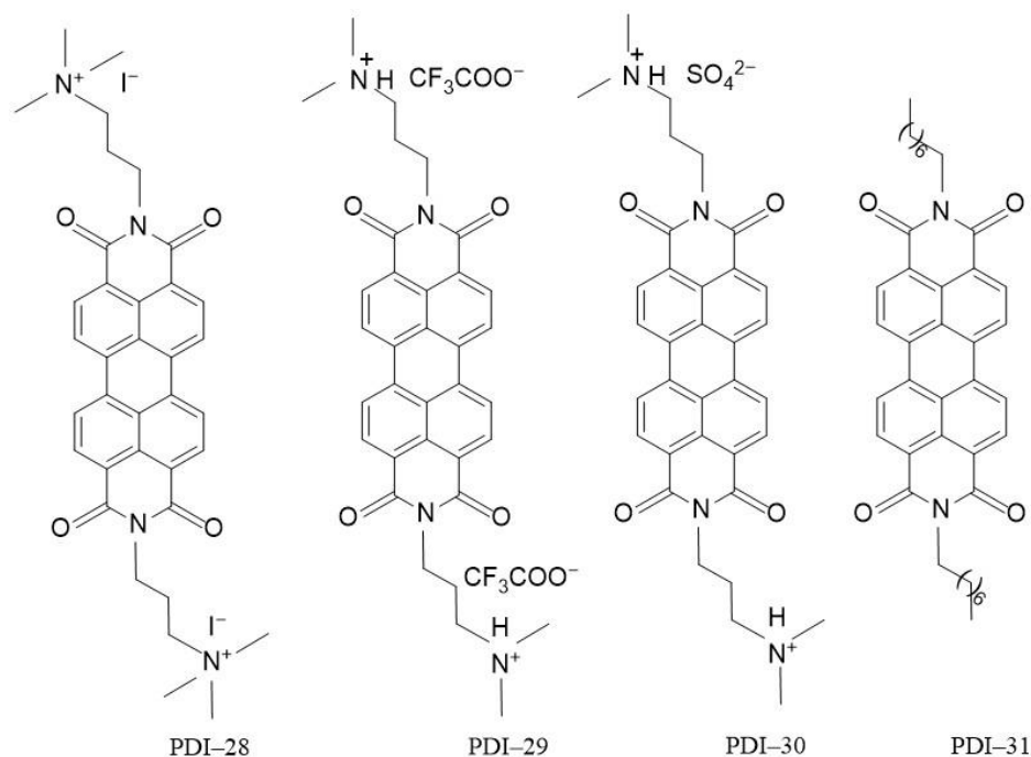
Figure 18. Molecular structures of PDI-28 to PDI-31.
