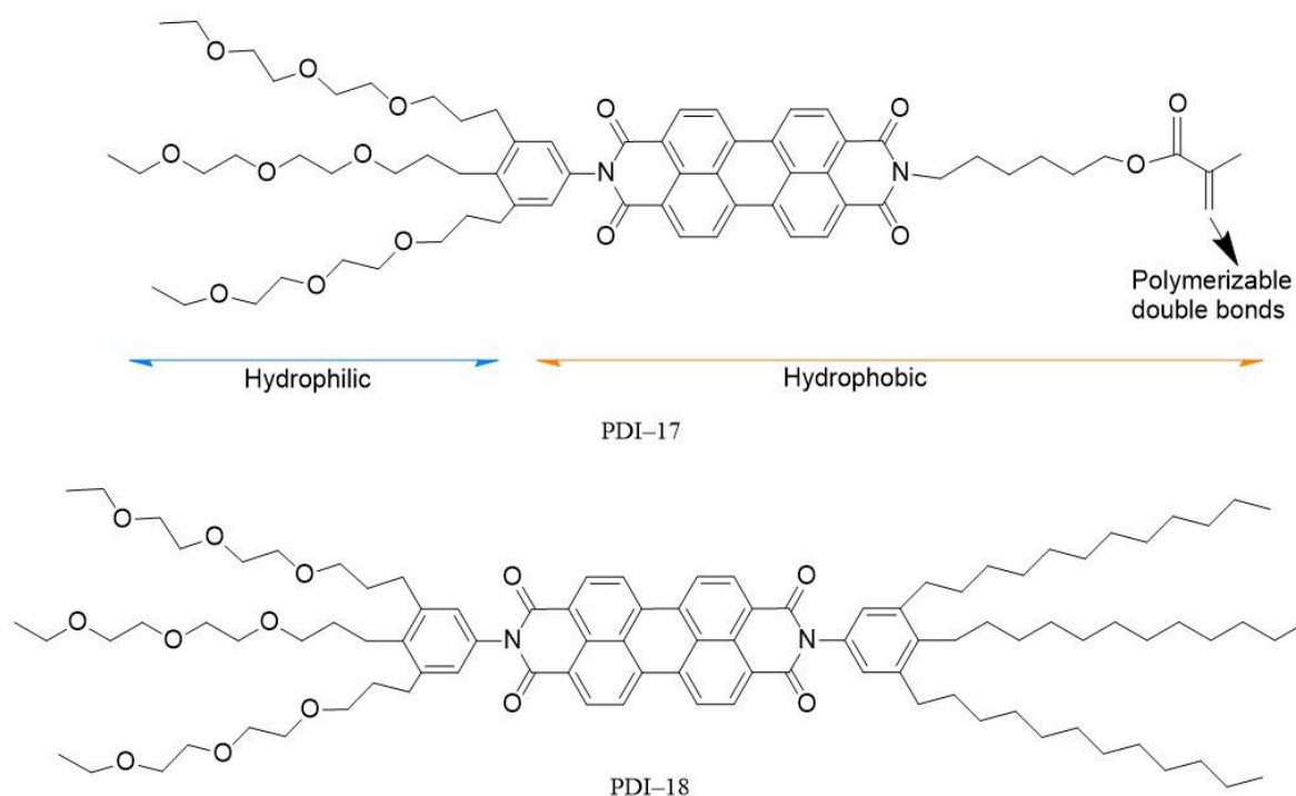
Figure 11. Molecular structures of PDI-17 and PDI-18.
