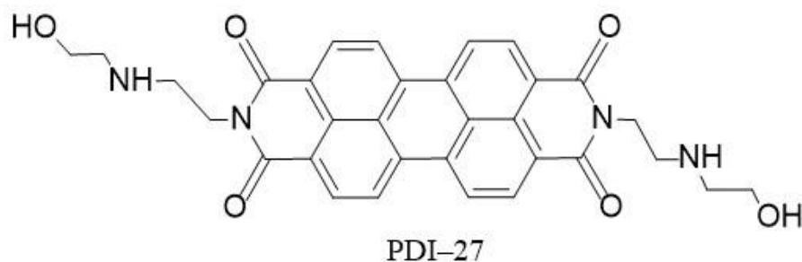
Figure 17. Molecular structure of PDI-27.
