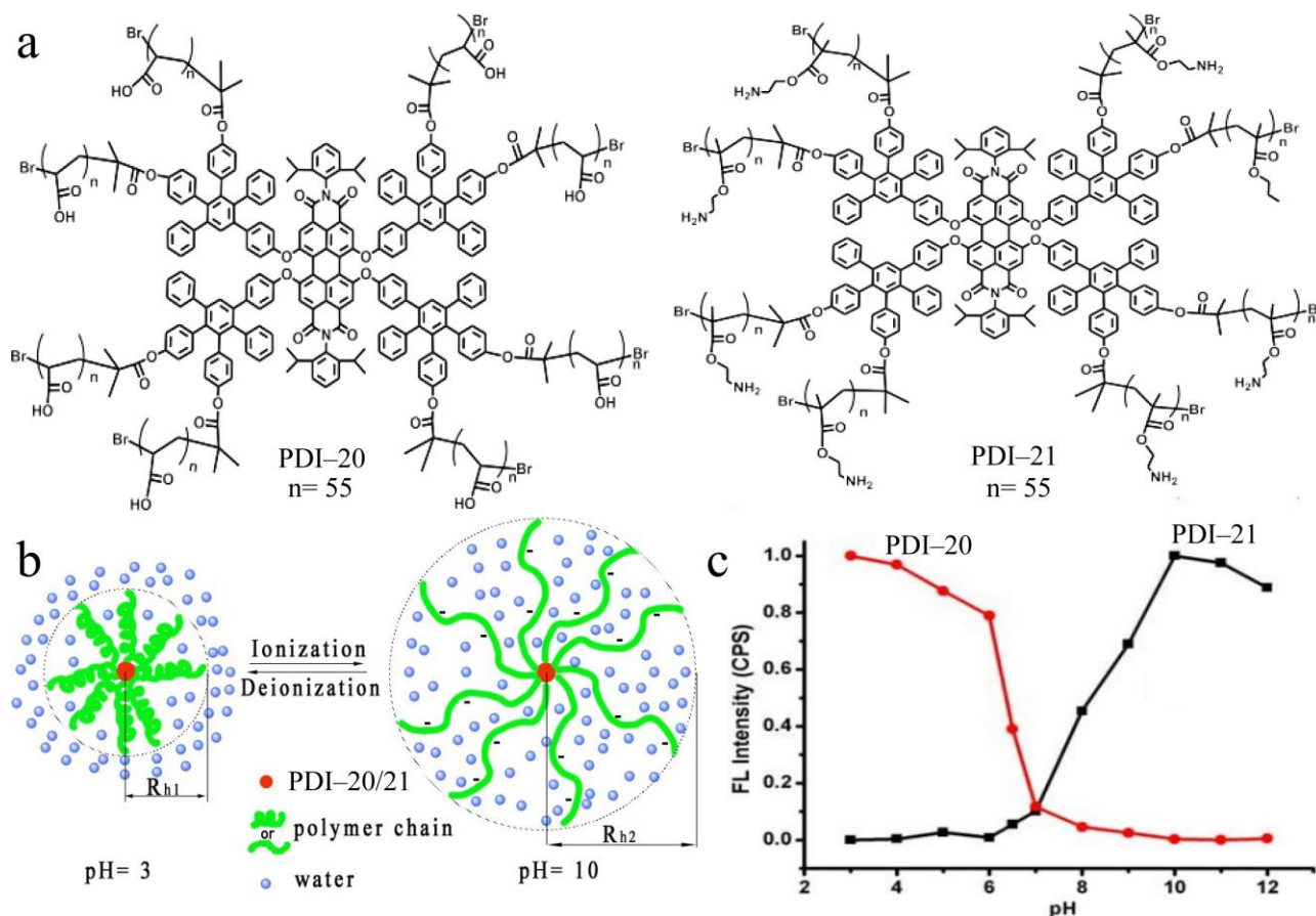
Figure 13. (a) Molecular structures of PDI-20 and PDI-21; (b) Schematic volume phase transition of PDI-20/21 unimolecular micelle; (c) Normalized peak fluorescence intensities (at \sim 620 nm for PDI-20 and \sim 607 nm for PDI-21) as a function of pH as tested in Tris-HCl buffer. Reproduced with permission from Ref [20].
